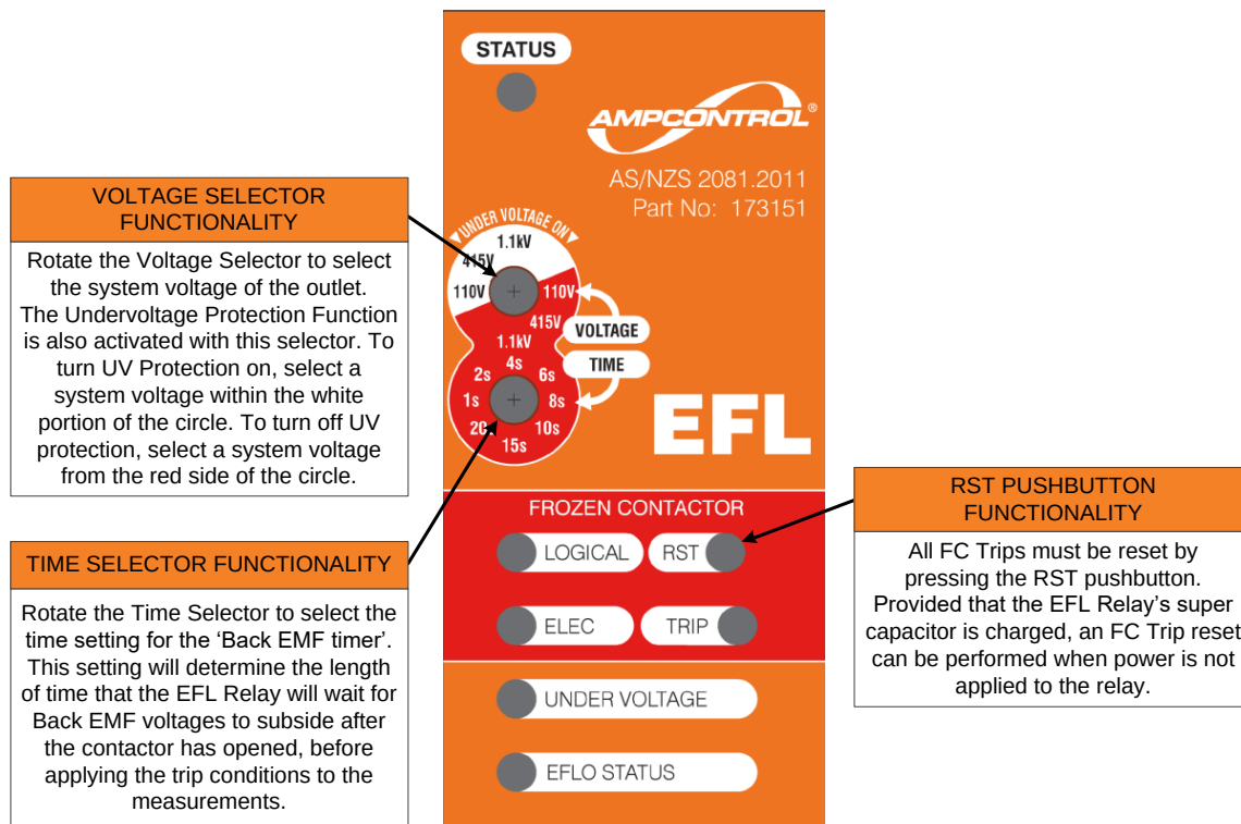
Figure 6.2: EFL Relay User Interface: Functionality of Operators
