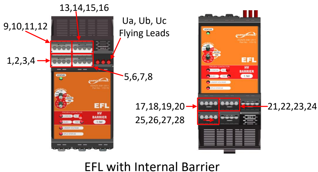
Figure 4.5: Terminal Numbering Arrangement for EFL Relay with Internal Barrier.
