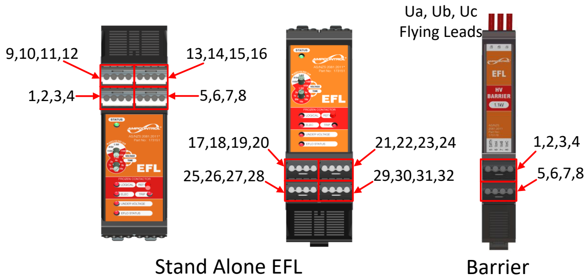
Figure 4.4: Terminal Numbering Arrangements for EFL Relay with External Barrier
