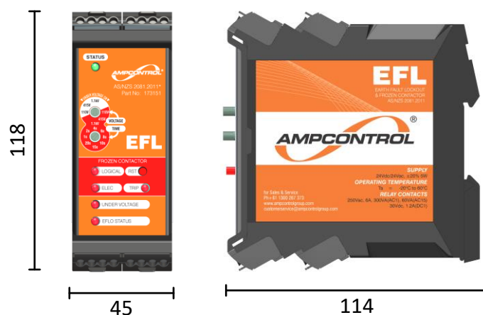
Figure 4.1: Enclosure Dimensions – Stand Alone EFL Relay
