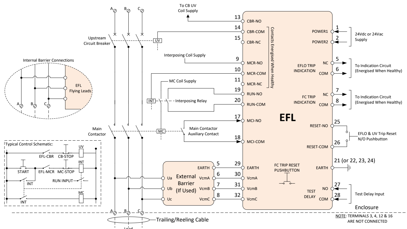
Figure 4.6: Typical Electrical Application
