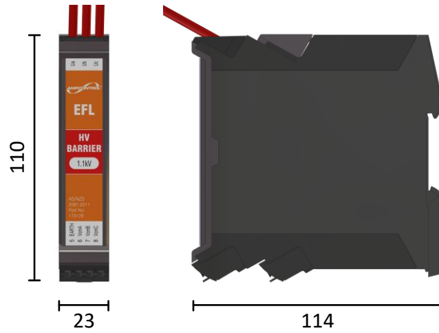
Figure 4.2: Enclosure Dimensions – External Barrier
