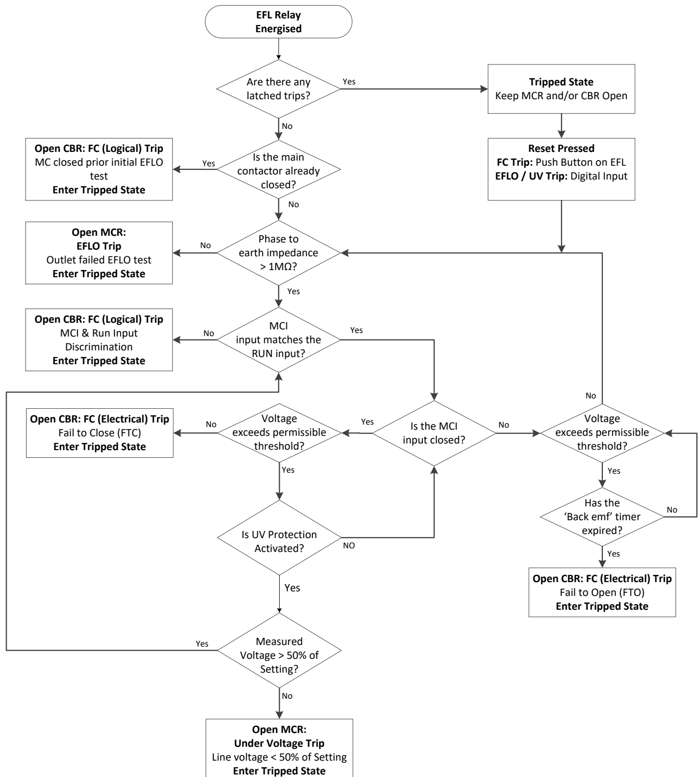
Figure 6.1: Logical Operation of the EFL Relay – General Overview
