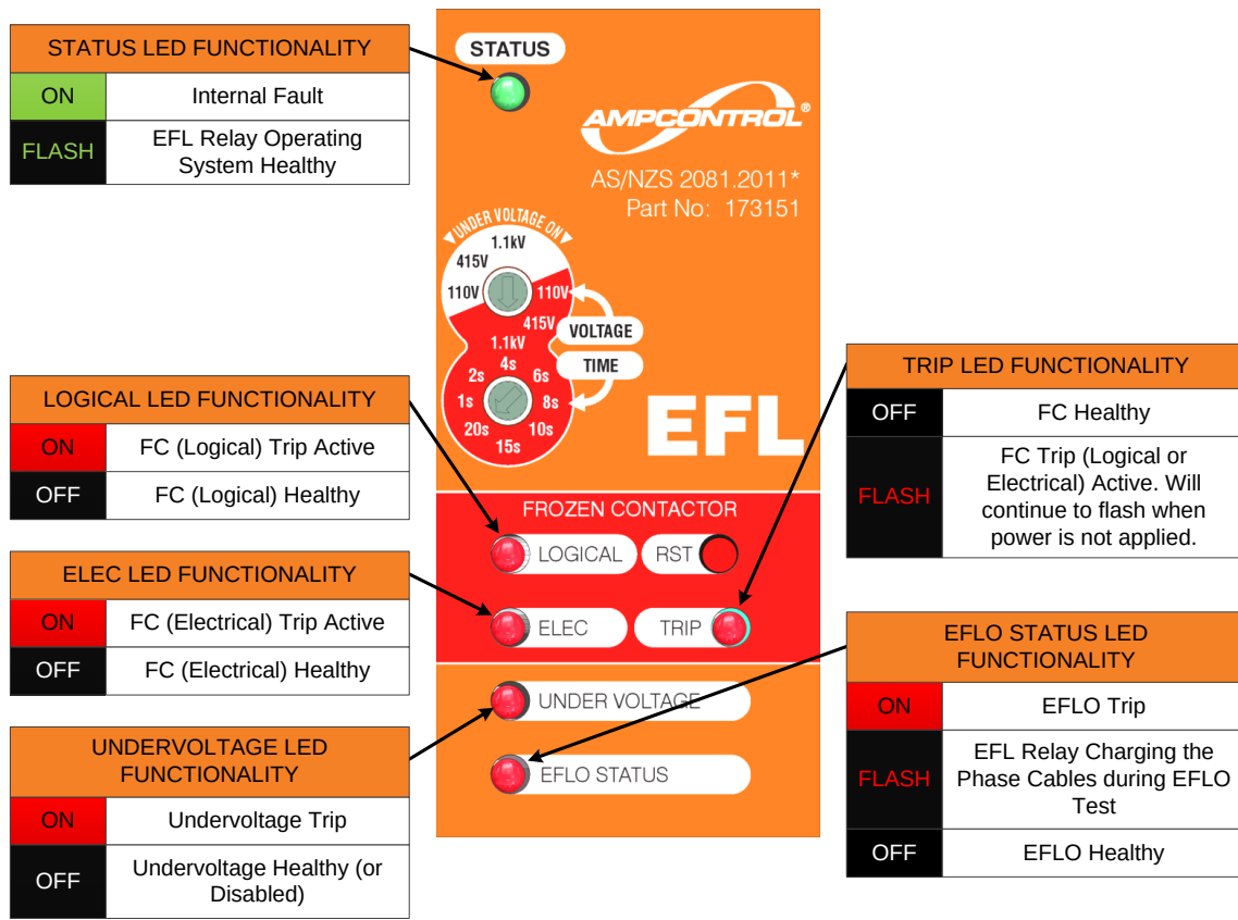
Figure 6.3: EFL Relay User Interface: Functionality of LEDs
